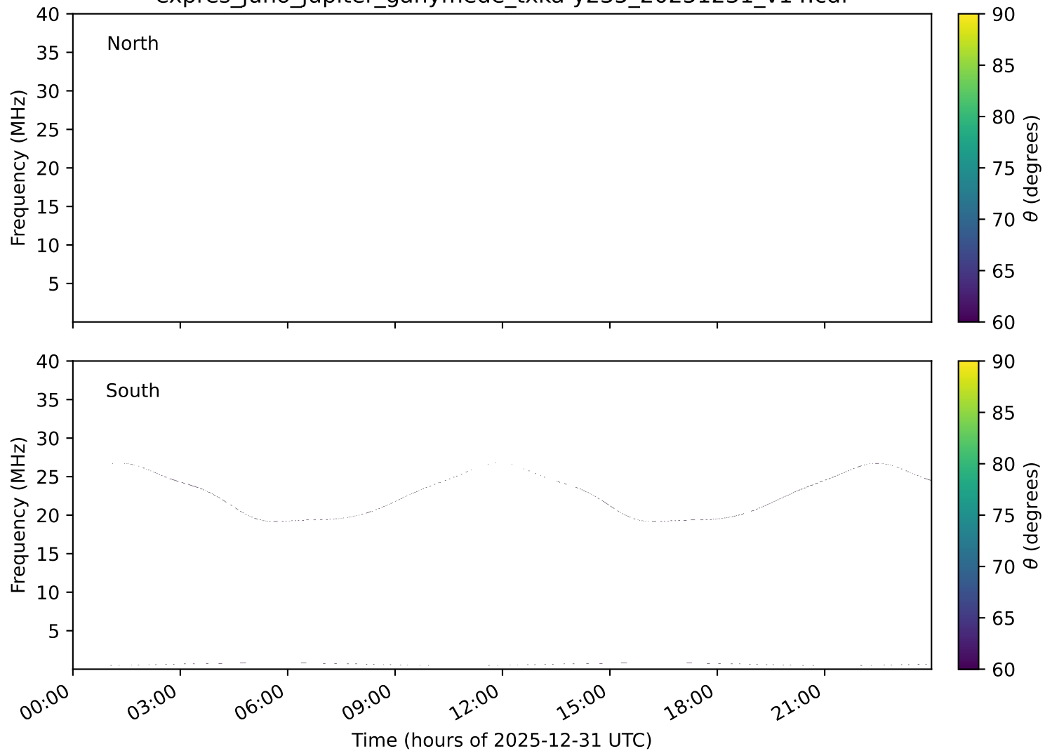
expres_juno_jupiter_ganymede_txka-y235_20251231_v14.cdf
