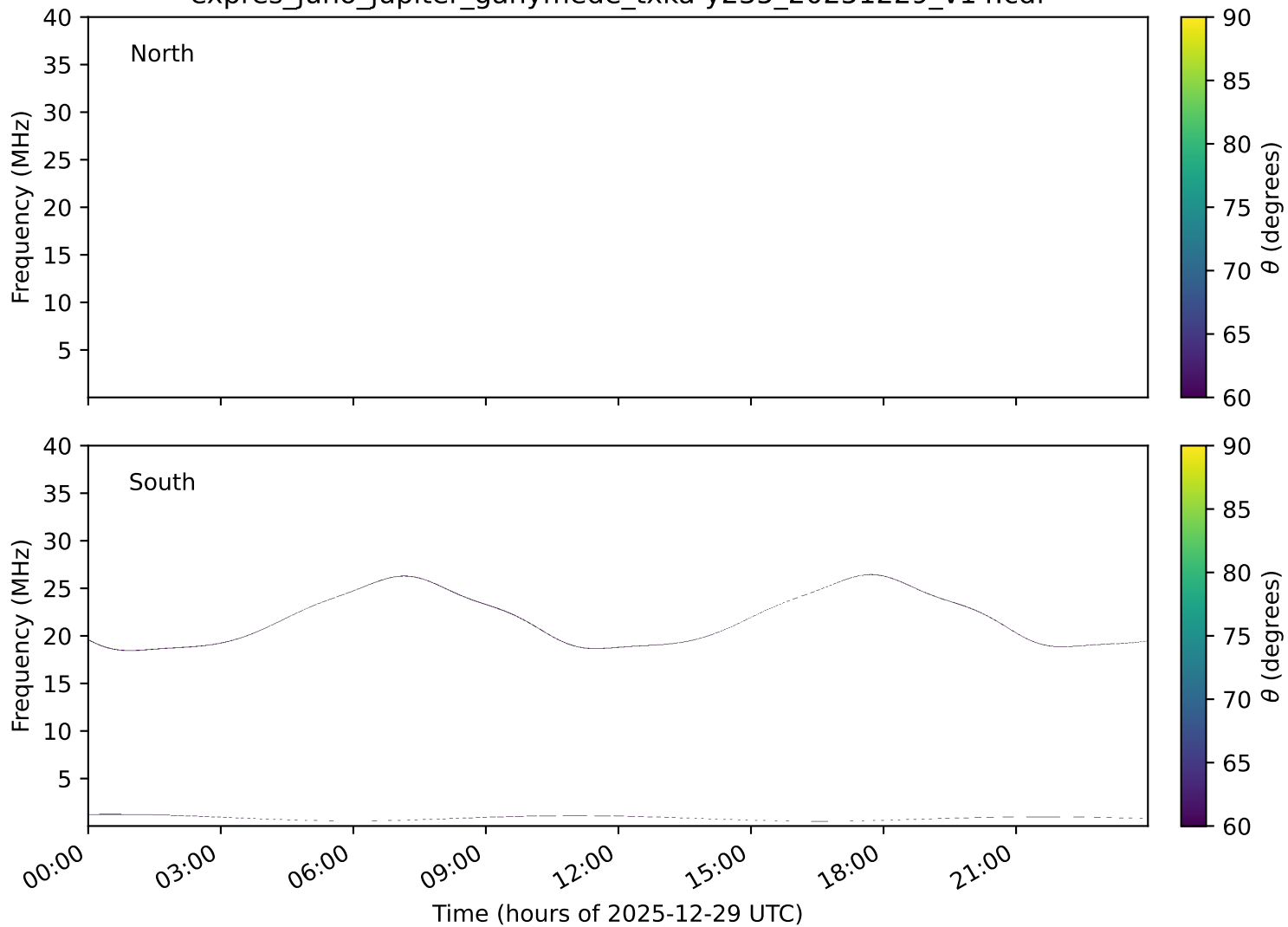
expres_juno_jupiter_ganymede_txka-y235_20251229_v14.cdf
