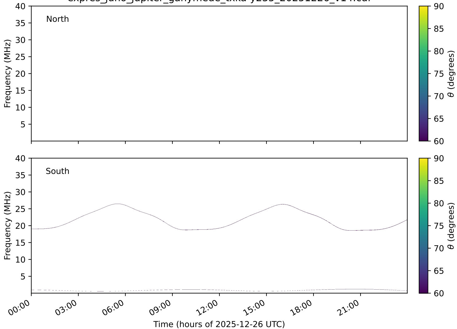
expres_juno_jupiter_ganymede_txka-y235_20251226_v14.cdf
