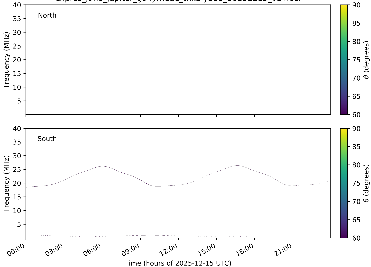
expres_juno_jupiter_ganymede_txka-y235_20251215_v14.cdf
