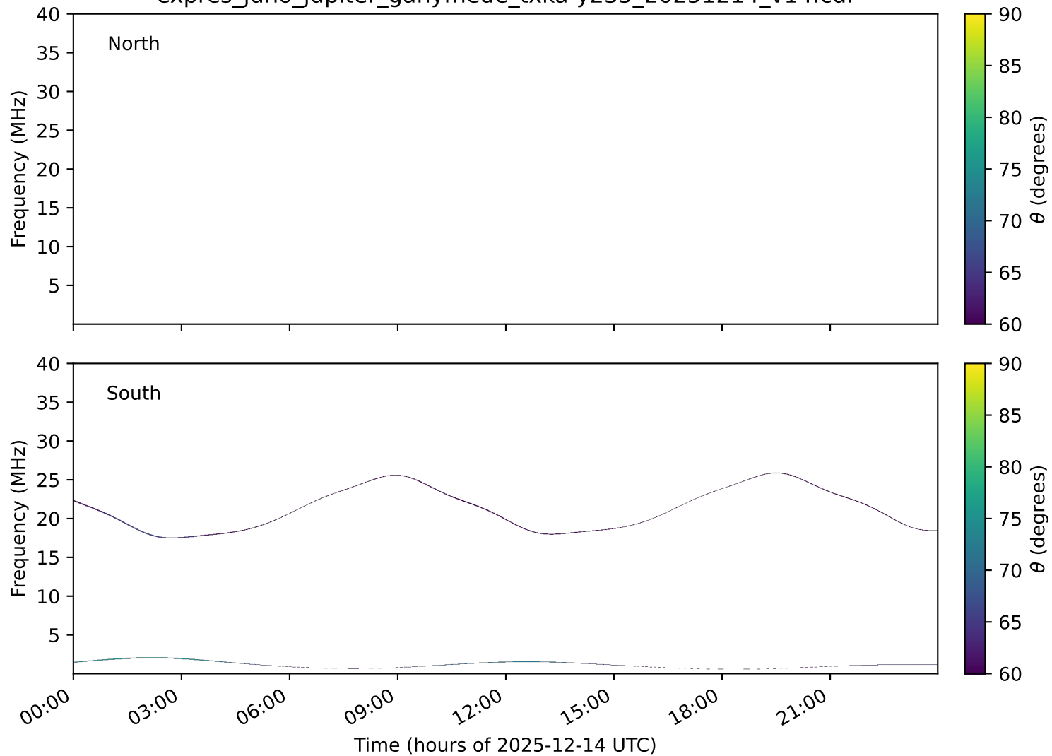
expres_juno_jupiter_ganymede_txka-y235_20251214_v14.cdf
