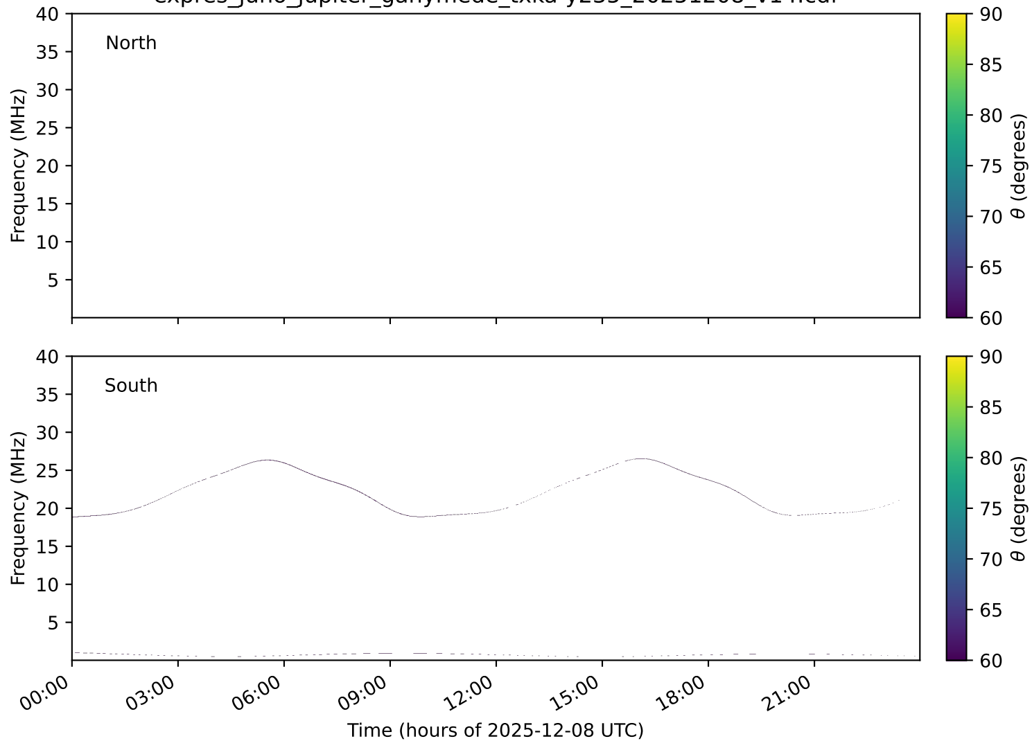
expres_juno_jupiter_ganymede_txka-y235_20251208_v14.cdf
