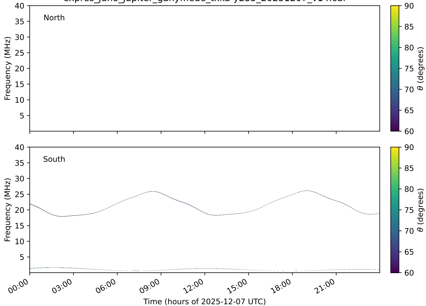
expres_juno_jupiter_ganymede_txka-y235_20251207_v14.cdf
