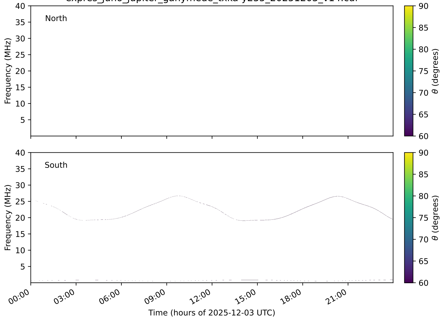
expres_juno_jupiter_ganymede_txka-y235_20251203_v14.cdf
