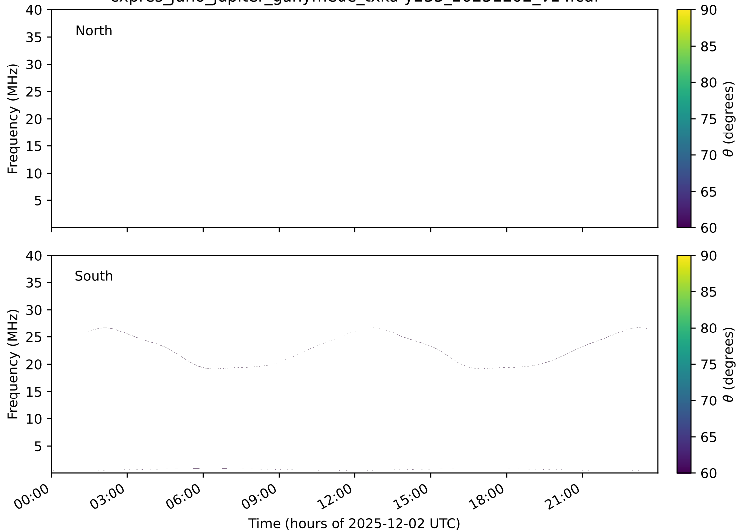
expres_juno_jupiter_ganymede_txka-y235_20251202_v14.cdf
