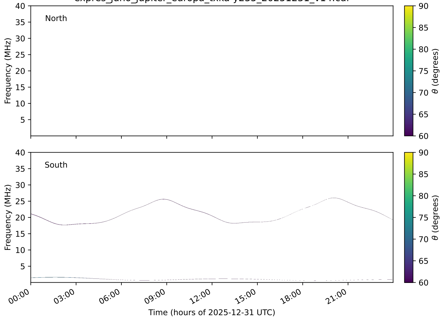
expres_juno_jupiter_europa_txka-y235_20251231_v14.cdf
