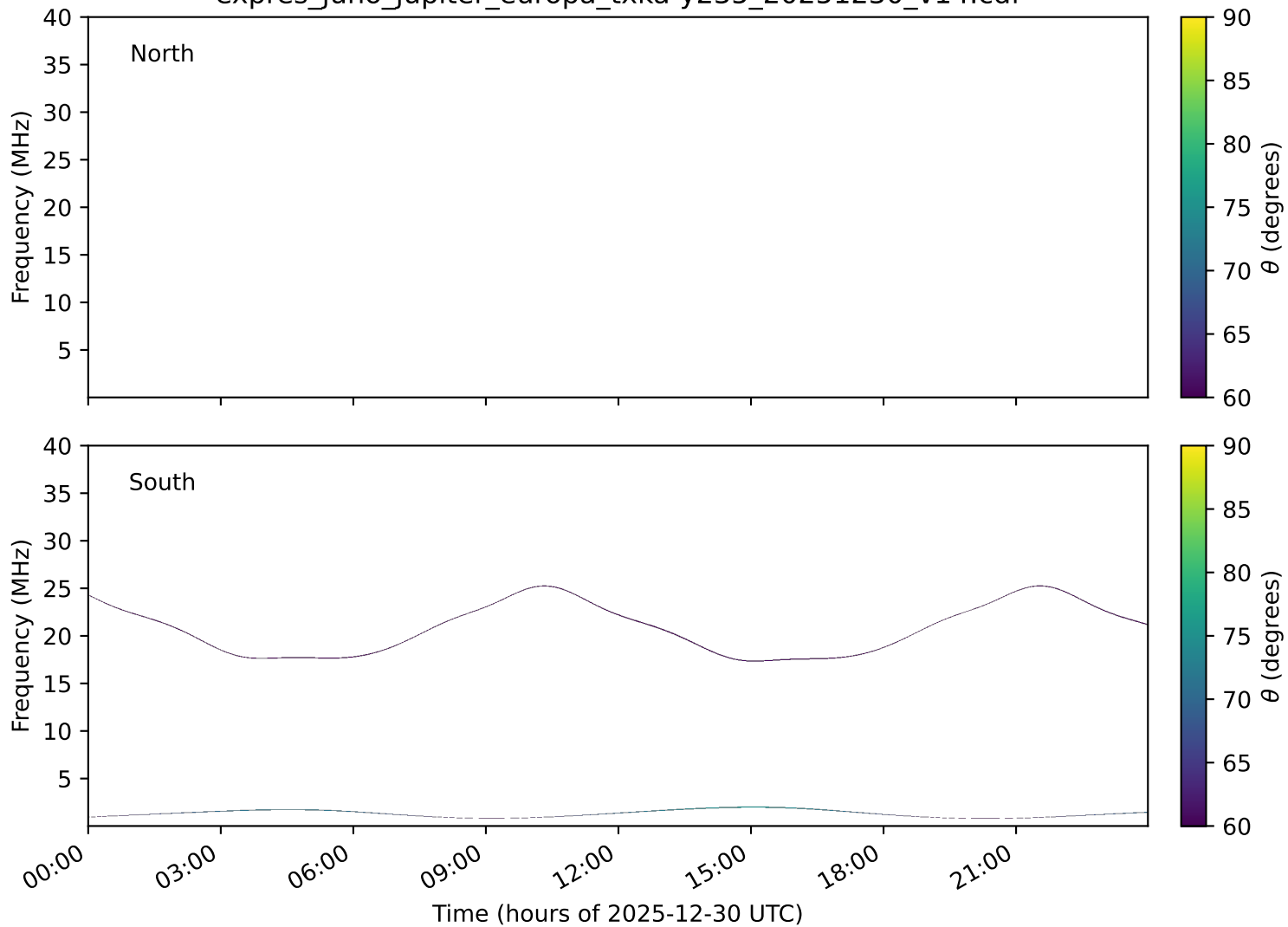
expres_juno_jupiter_europa_txka-y235_20251230_v14.cdf
