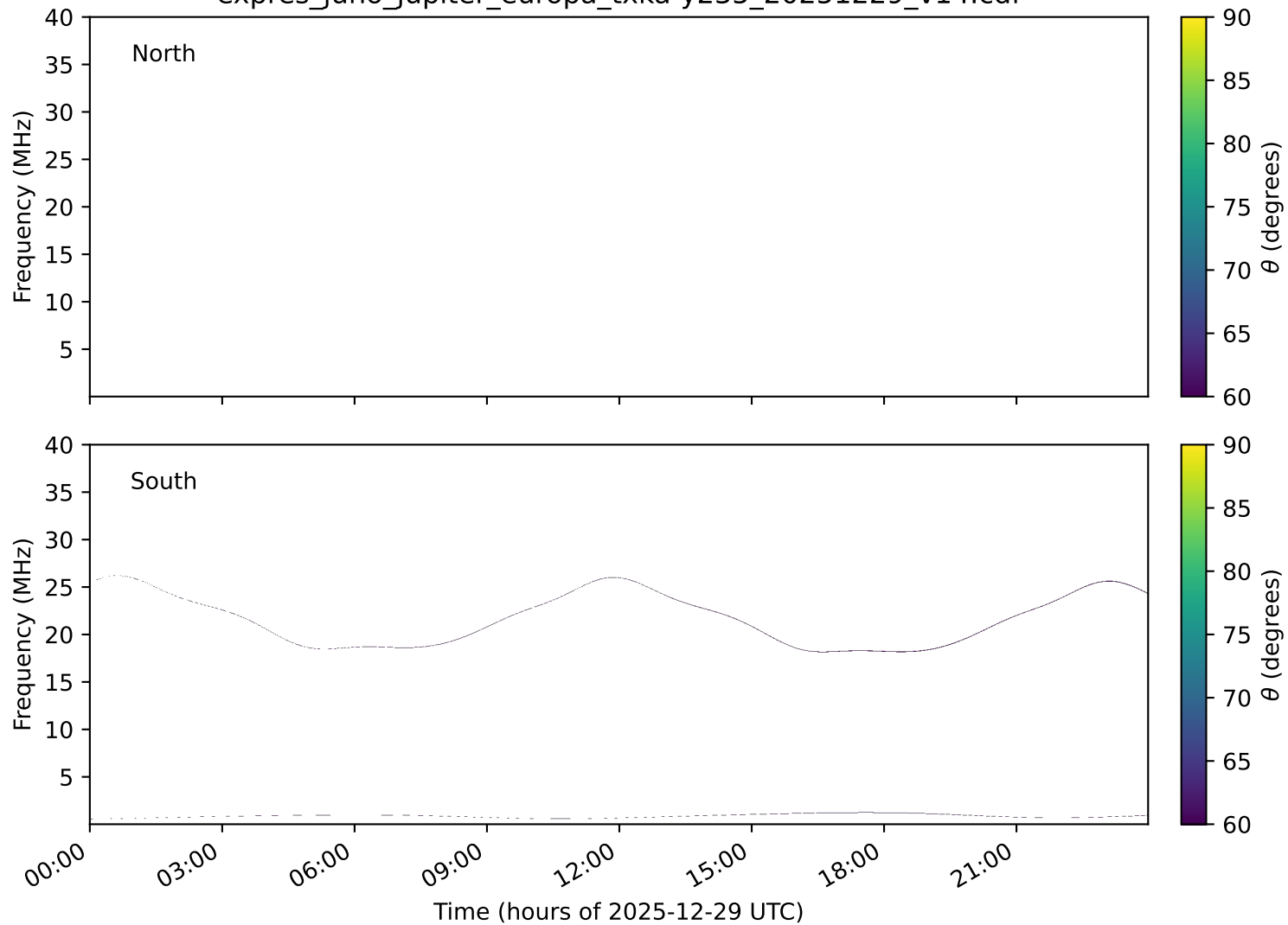
expres_juno_jupiter_europa_txka-y235_20251229_v14.cdf
