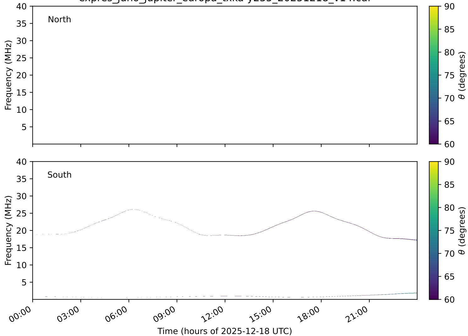
expres_juno_jupiter_europa_txka-y235_20251218_v14.cdf
