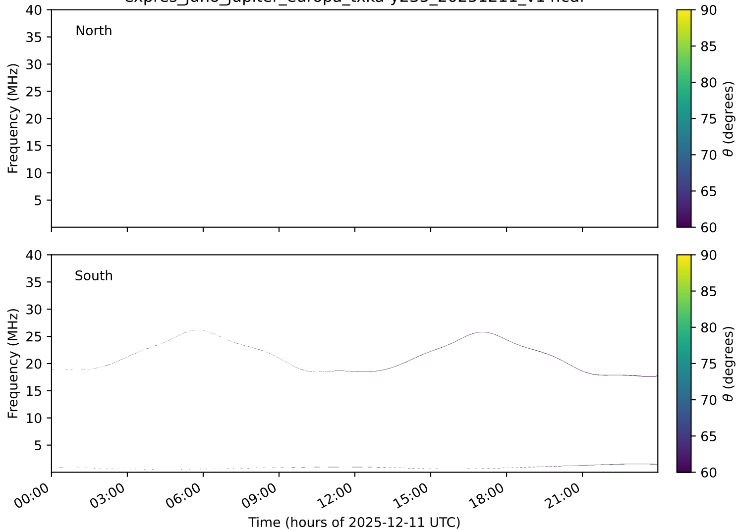
expres_juno_jupiter_europa_txka-y235_20251211_v14.cdf
