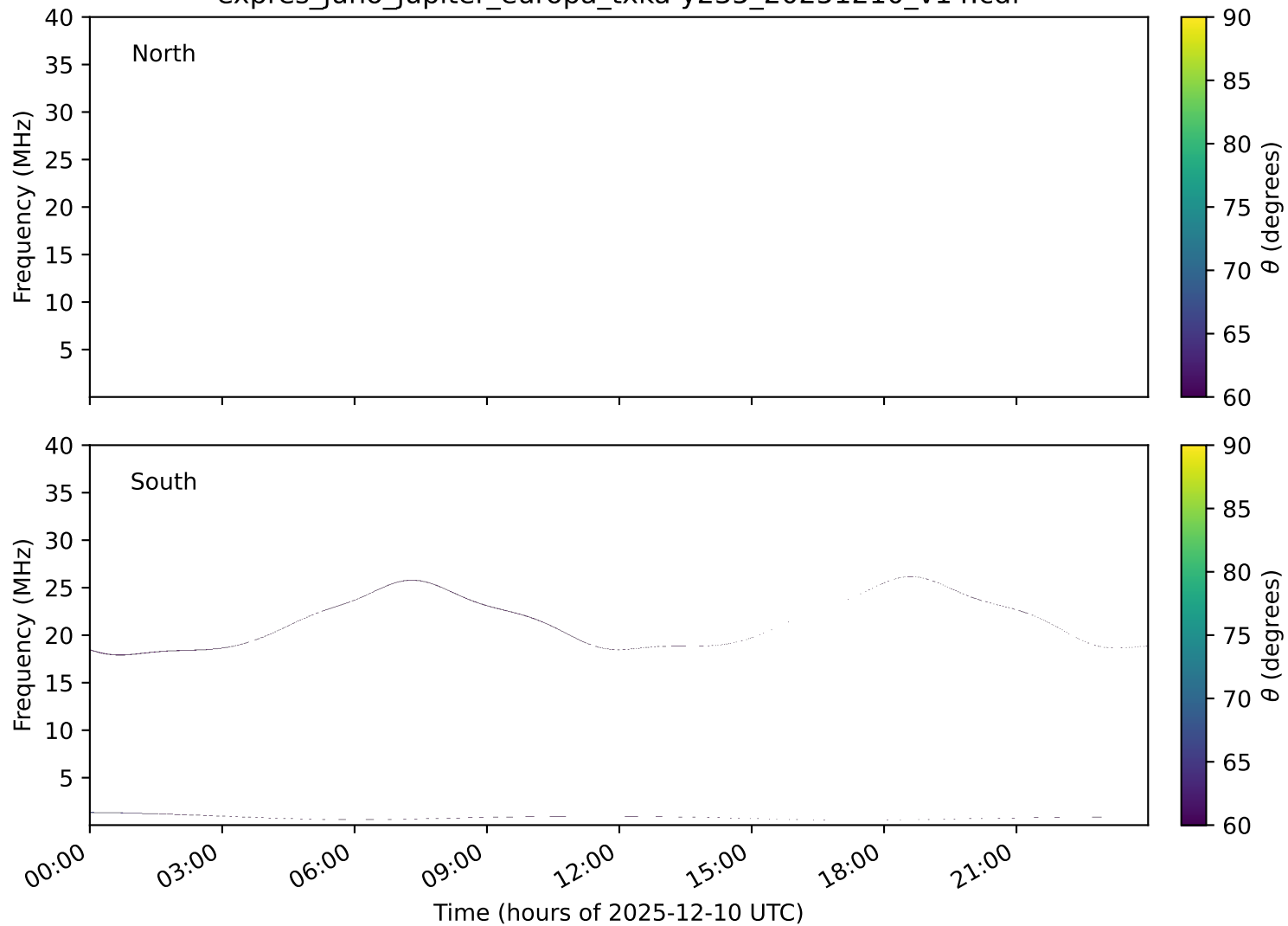
expres_juno_jupiter_europa_txka-y235_20251210_v14.cdf
