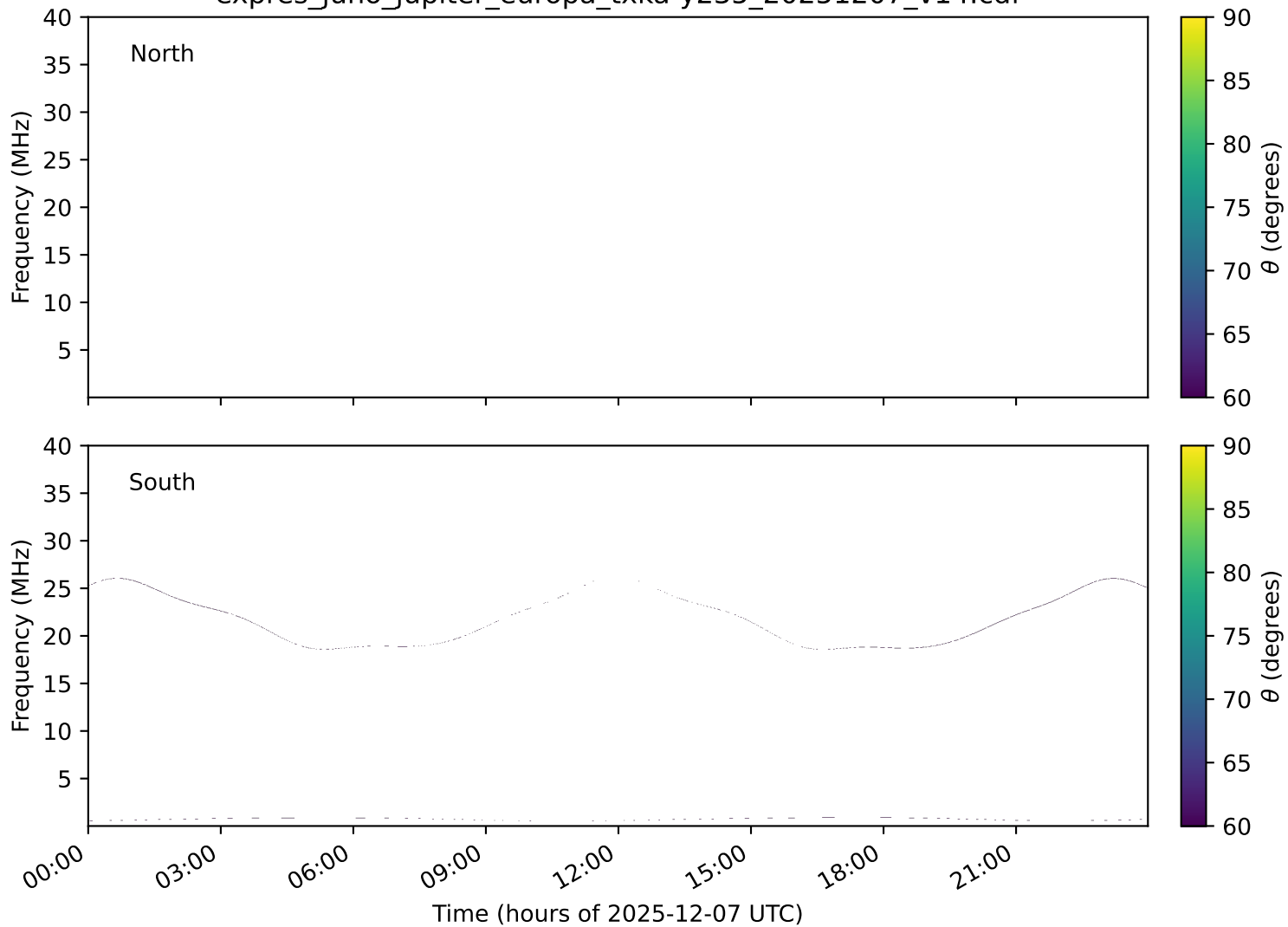
expres_juno_jupiter_europa_txka-y235_20251207_v14.cdf
