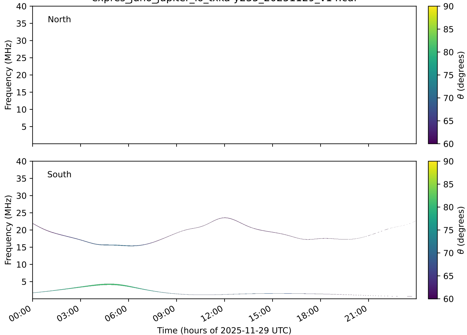
expres_juno_jupiter_io_txka-y235_20251129_v14.cdf
