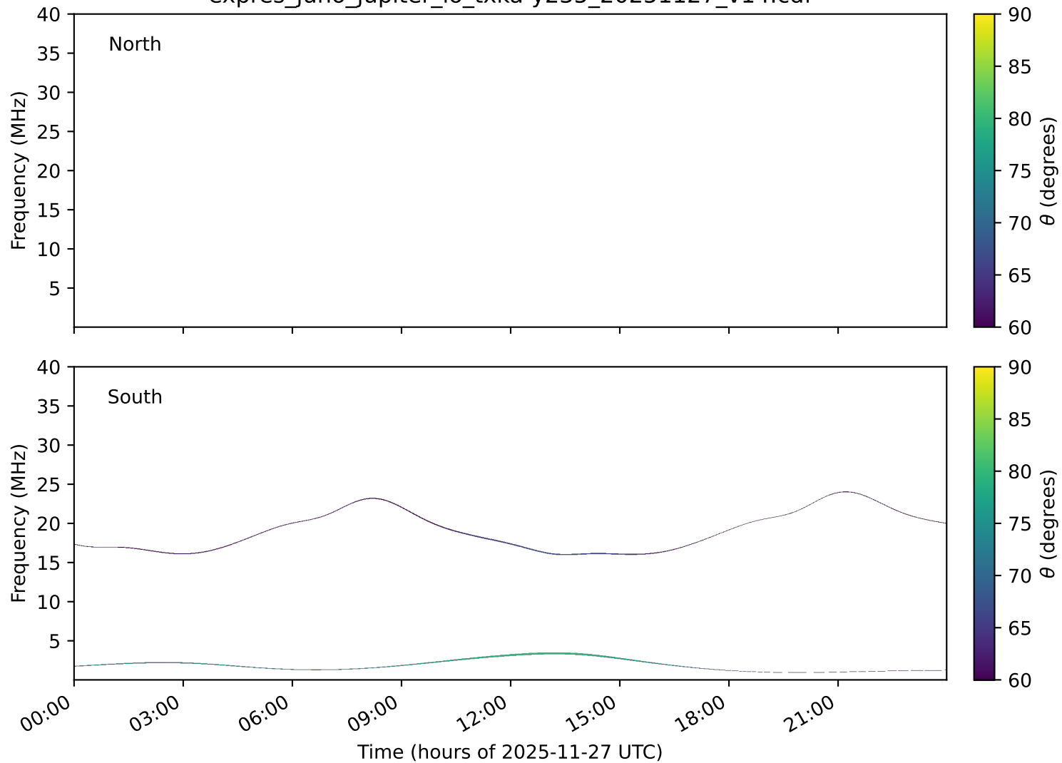
expres_juno_jupiter_io_txka-y235_20251127_v14.cdf
