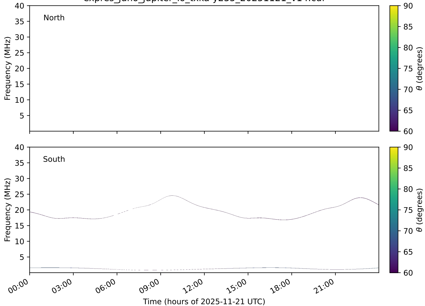
expres_juno_jupiter_io_txka-y235_20251121_v14.cdf
