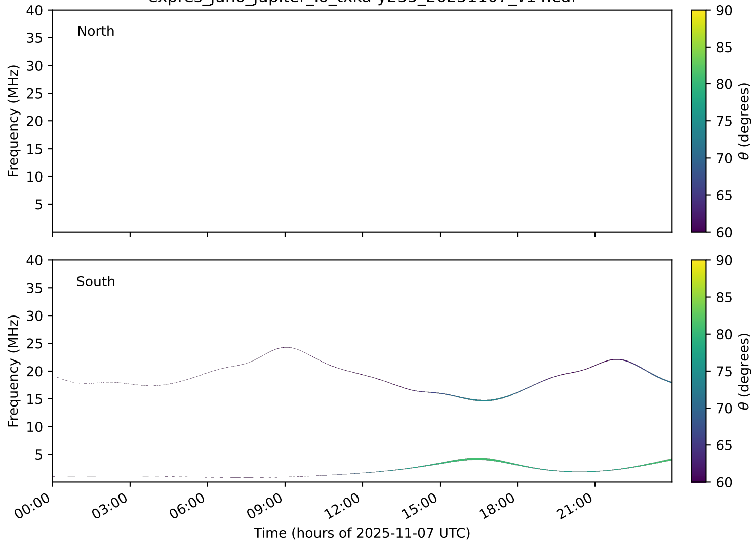
expres_juno_jupiter_io_txka-y235_20251107_v14.cdf
