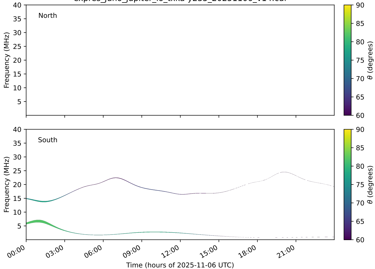
expres_juno_jupiter_io_txka-y235_20251106_v14.cdf
