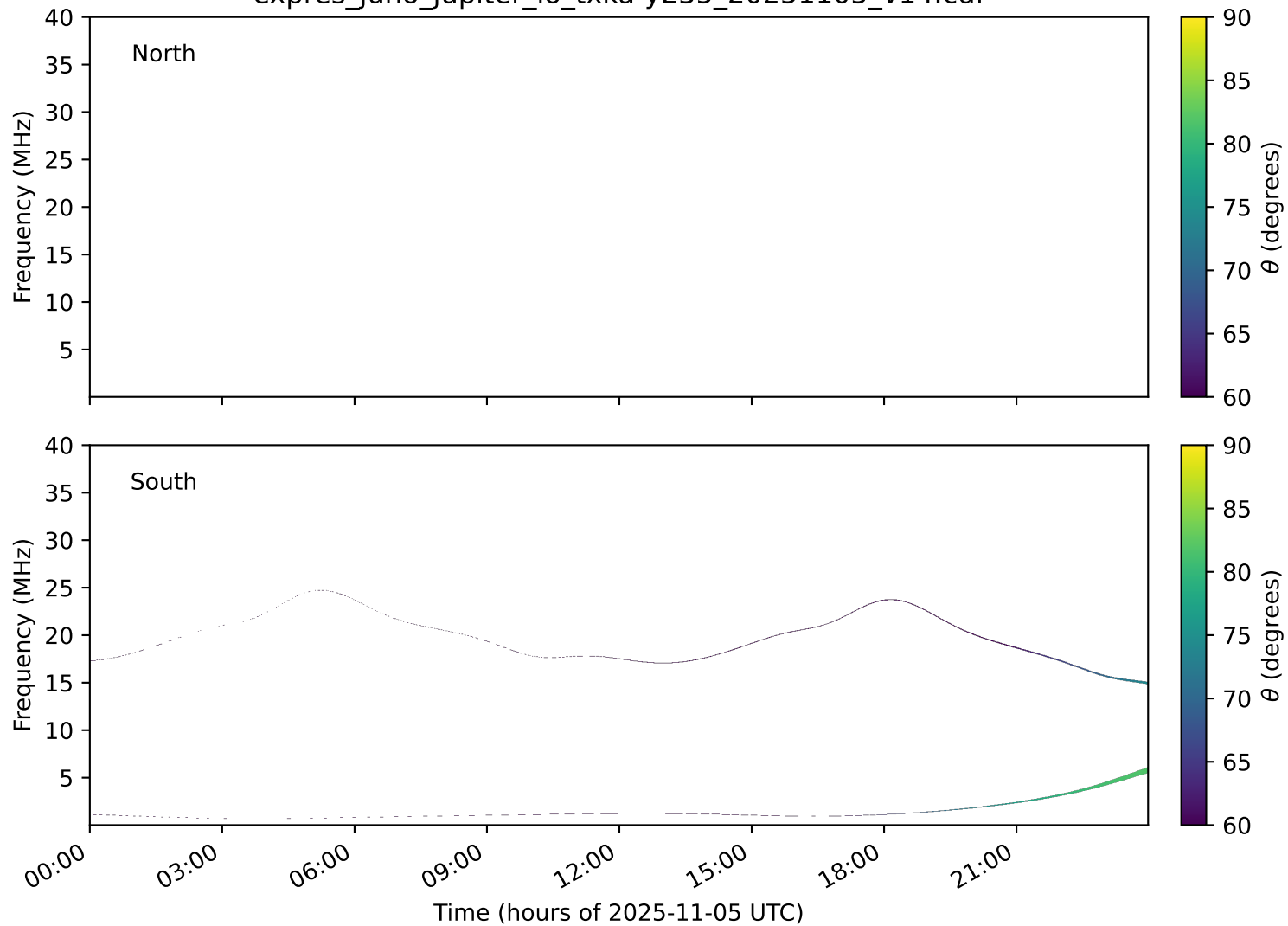
expres_juno_jupiter_io_txka-y235_20251105_v14.cdf
