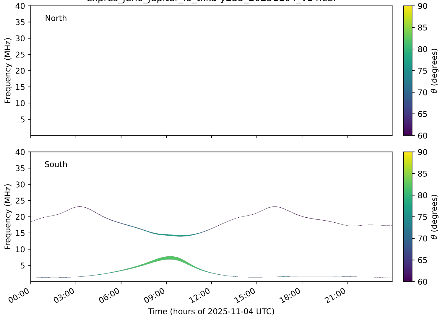
expres_juno_jupiter_io_txka-y235_20251104_v14.cdf
