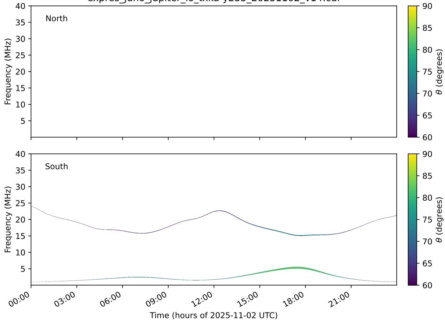
expres_juno_jupiter_io_txka-y235_20251102_v14.cdf
