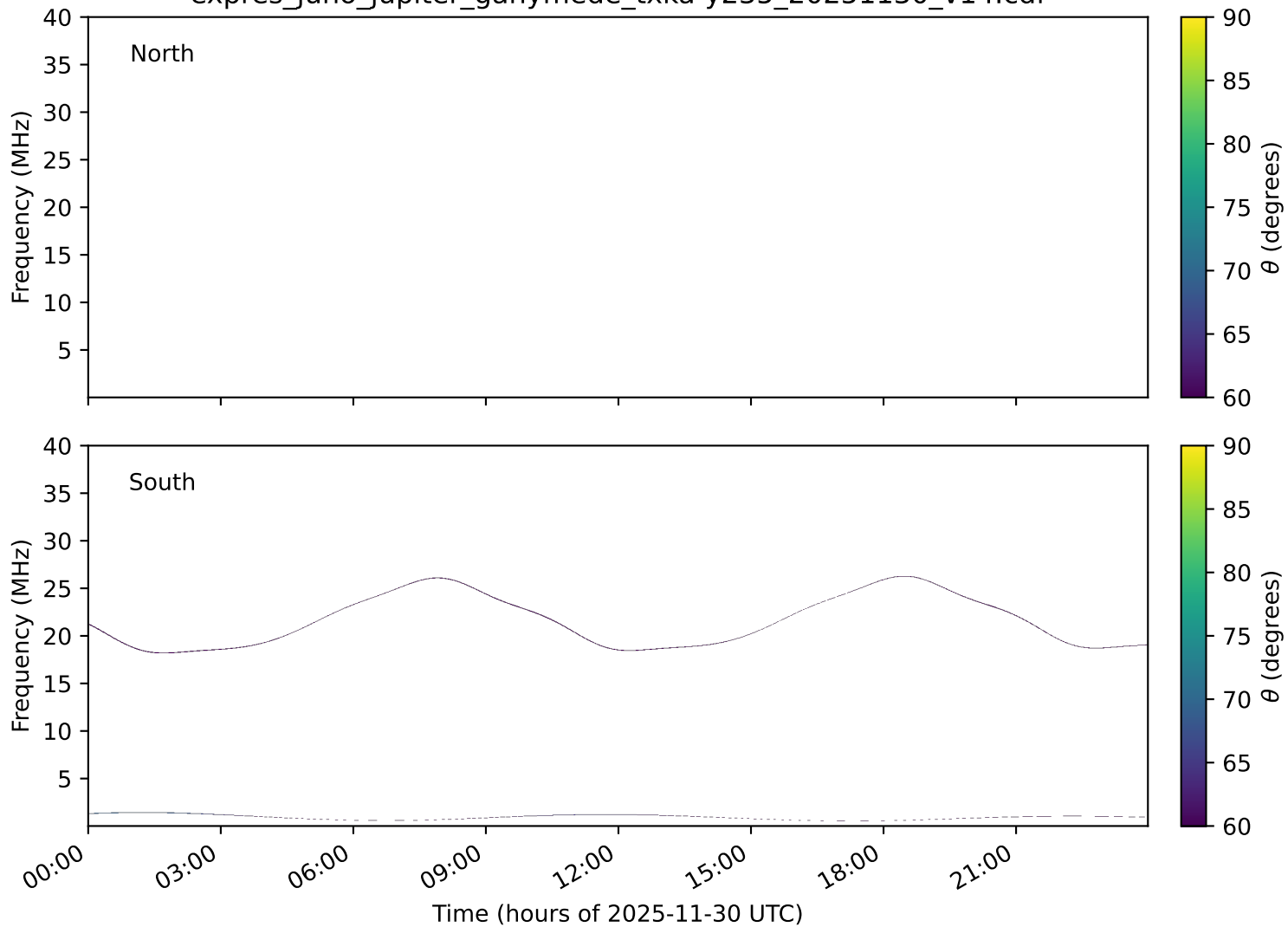
expres_juno_jupiter_ganymede_txka-y235_20251130_v14.cdf
