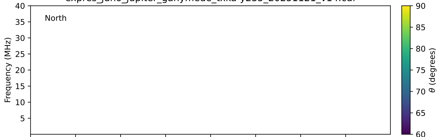
expres_juno_jupiter_ganymede_txka-y235_20251121_v14.cdf
