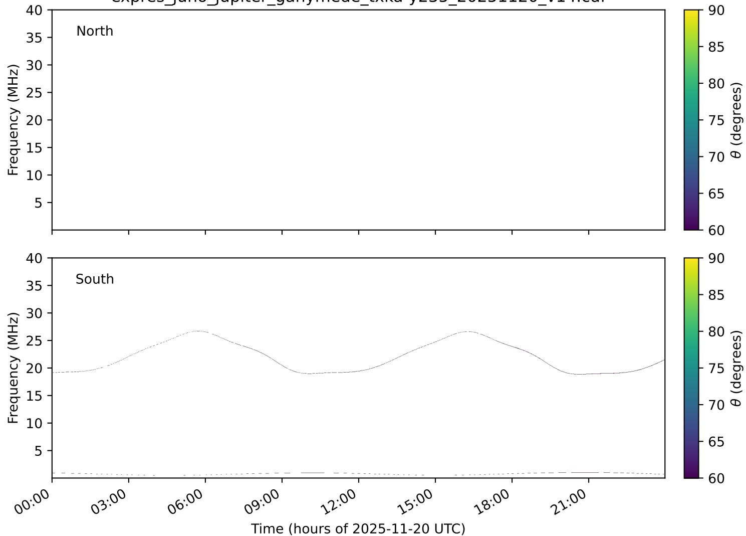
expres_juno_jupiter_ganymede_txka-y235_20251120_v14.cdf
