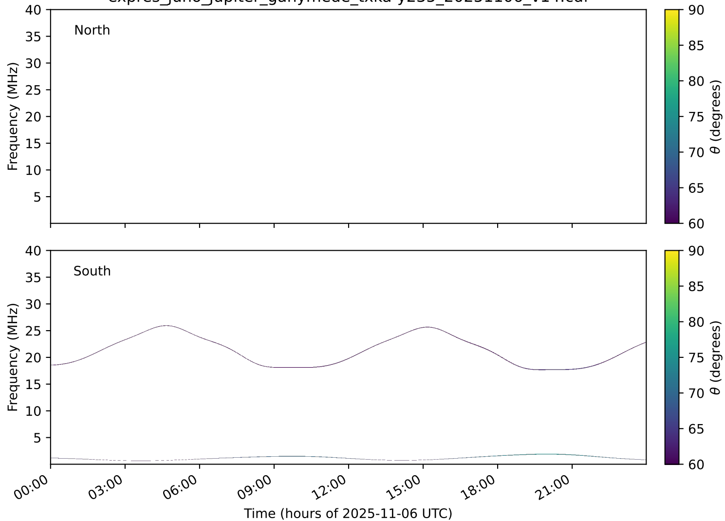
expres_juno_jupiter_ganymede_txka-y235_20251106_v14.cdf
