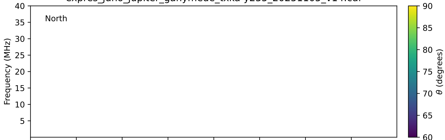
expres_juno_jupiter_ganymede_txka-y235_20251105_v14.cdf
