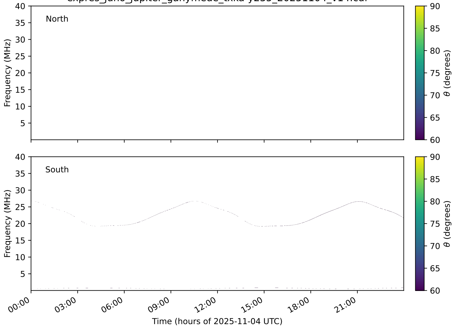
expres_juno_jupiter_ganymede_txka-y235_20251104_v14.cdf
