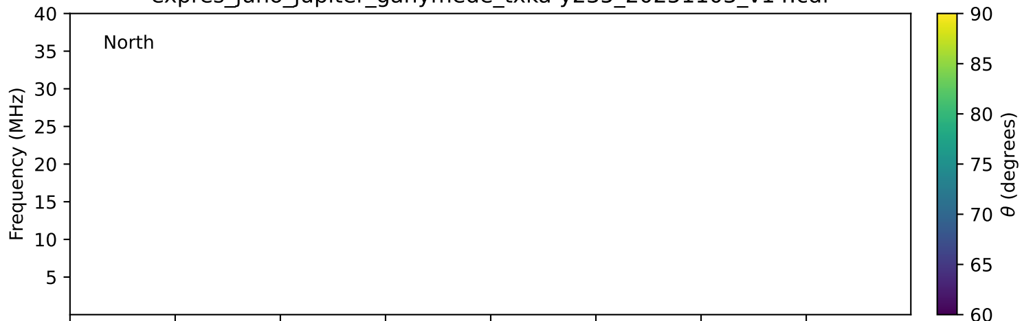
expres_juno_jupiter_ganymede_txka-y235_20251103_v14.cdf
