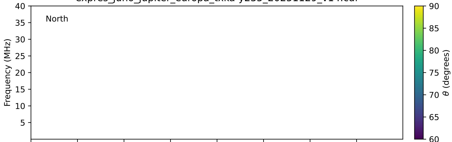
expres_juno_jupiter_europa_txka-y235_20251129_v14.cdf
