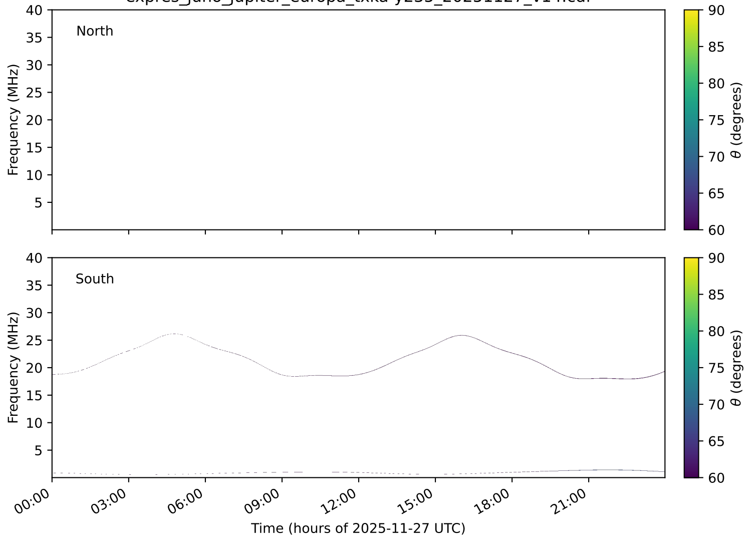
expres_juno_jupiter_europa_txka-y235_20251127_v14.cdf
