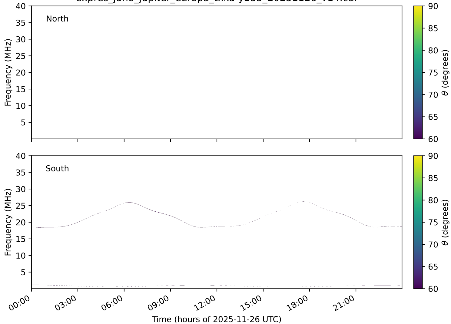
expres_juno_jupiter_europa_txka-y235_20251126_v14.cdf
