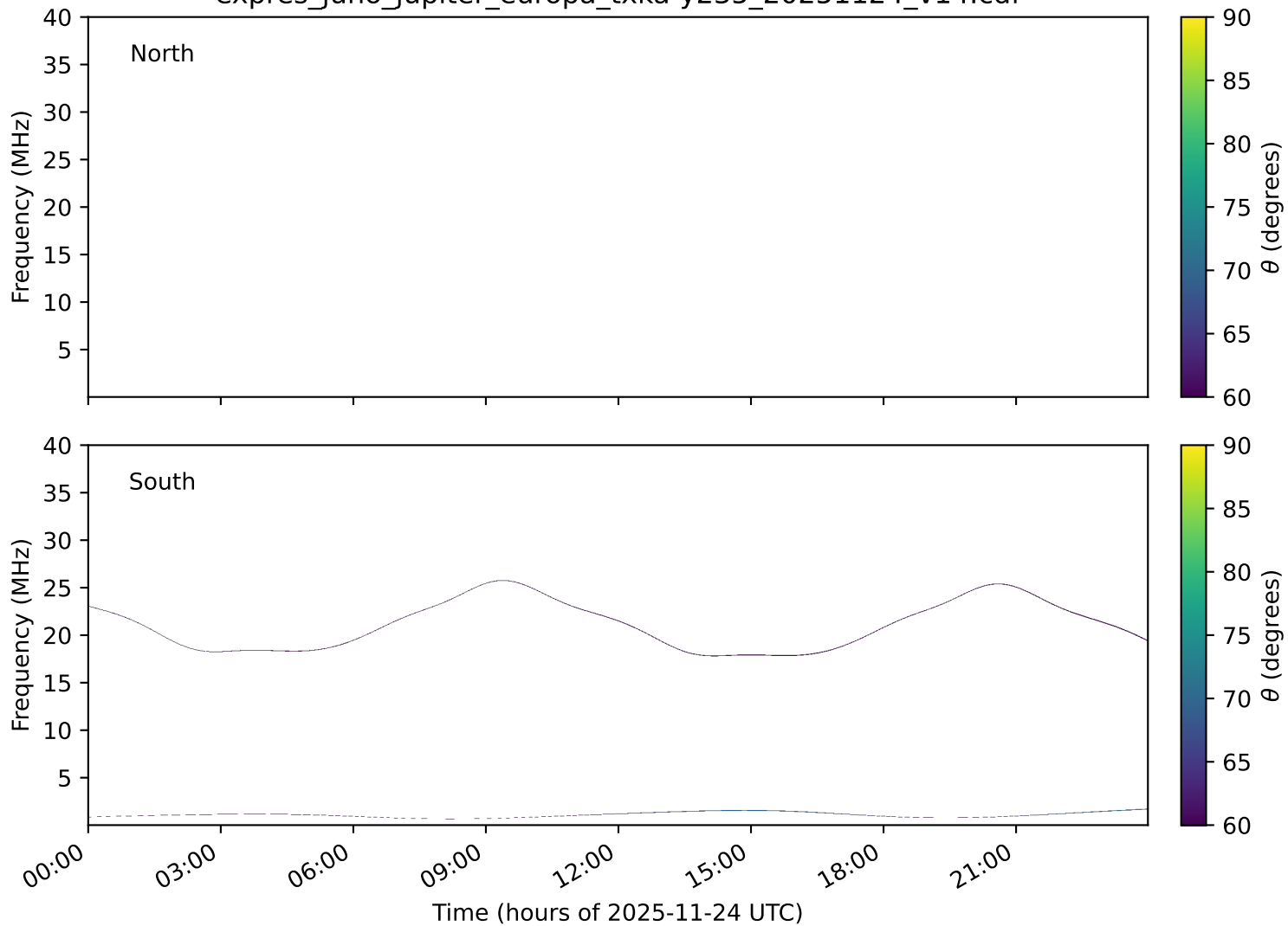
expres_juno_jupiter_europa_txka-y235_20251124_v14.cdf
