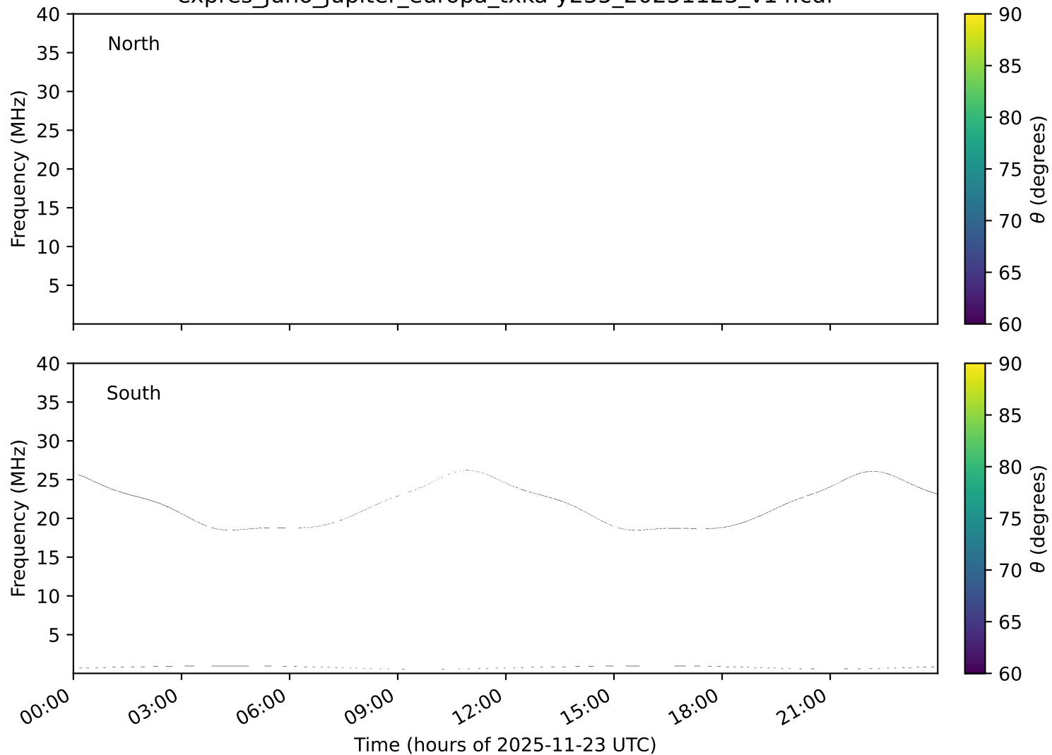
expres_juno_jupiter_europa_txka-y235_20251123_v14.cdf
