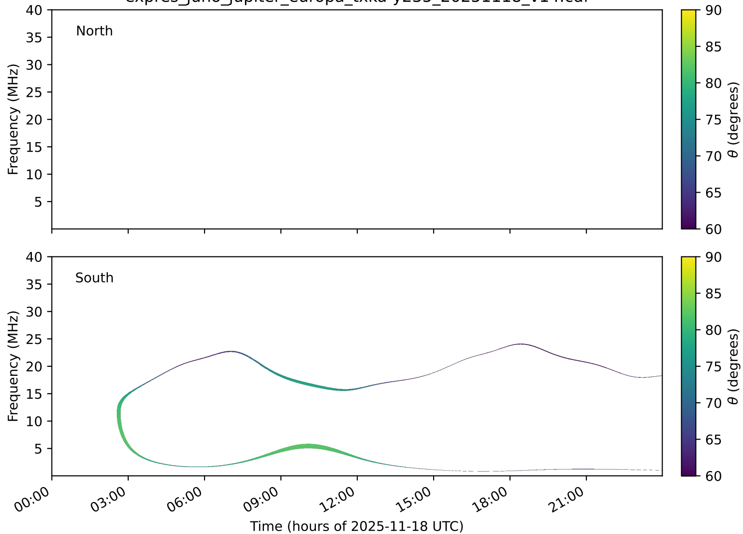
expres_juno_jupiter_europa_txka-y235_20251118_v14.cdf
