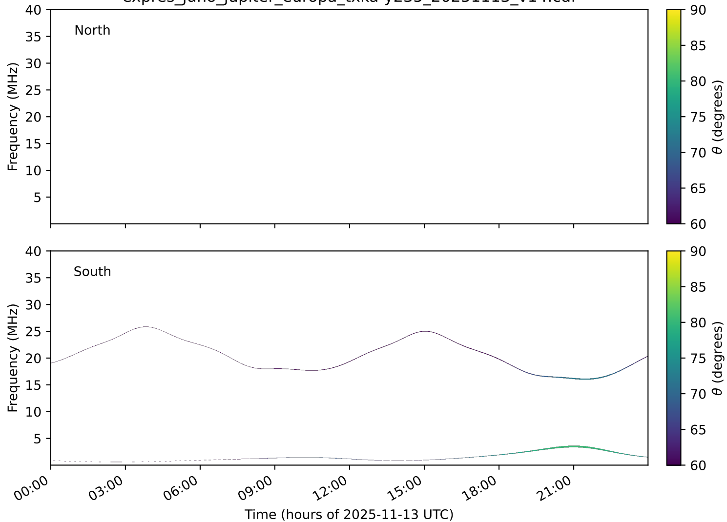
expres_juno_jupiter_europa_txka-y235_20251113_v14.cdf
