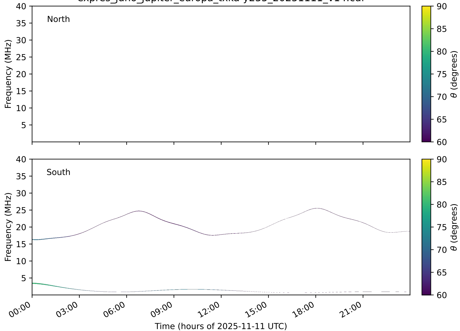
expres_juno_jupiter_europa_txka-y235_20251111_v14.cdf
