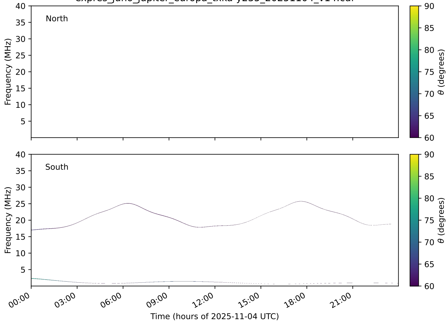
expres_juno_jupiter_europa_txka-y235_20251104_v14.cdf
