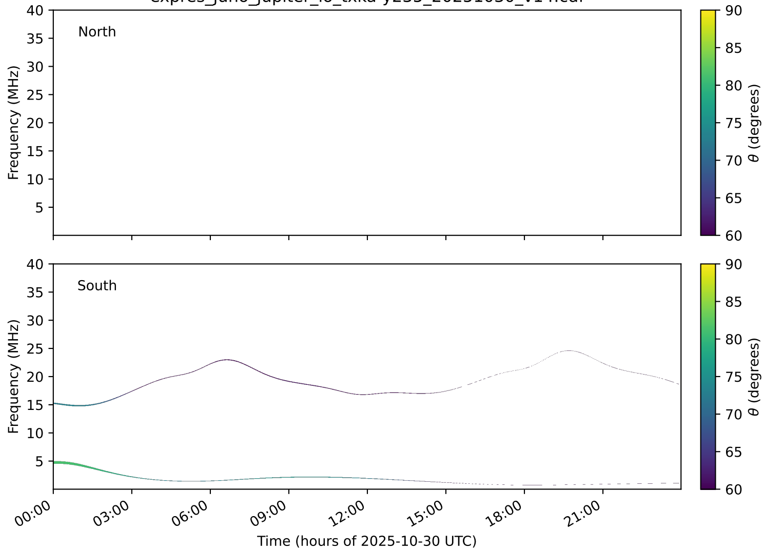
expres_juno_jupiter_io_txka-y235_20251030_v14.cdf
