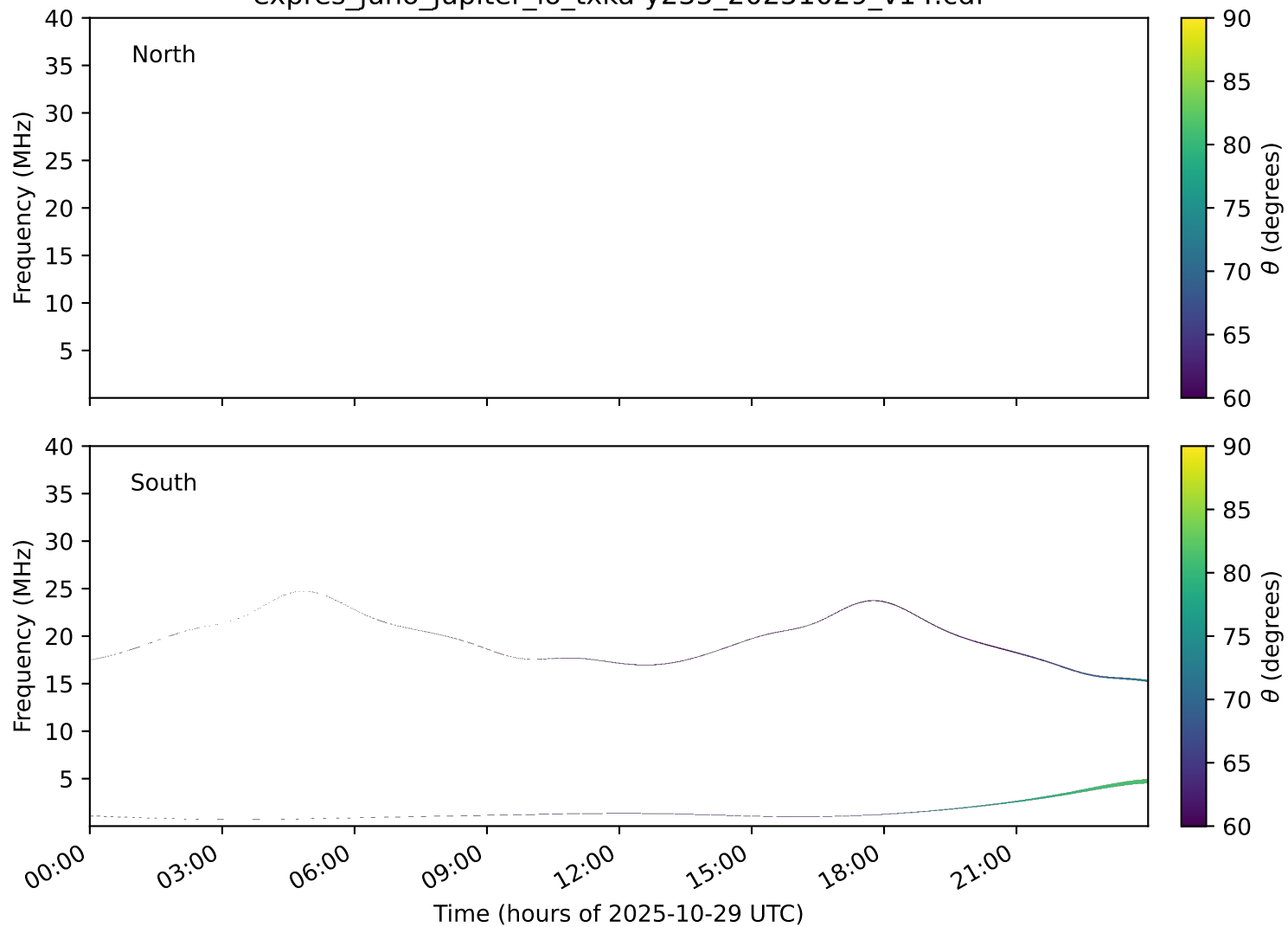
expres_juno_jupiter_io_txka-y235_20251029_v14.cdf
