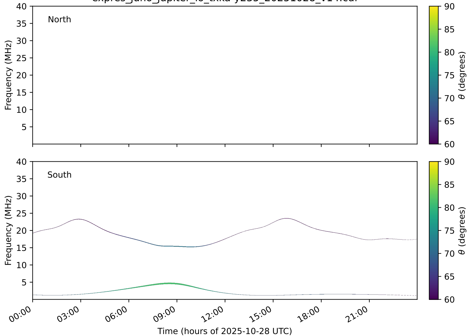
expres_juno_jupiter_io_txka-y235_20251028_v14.cdf
