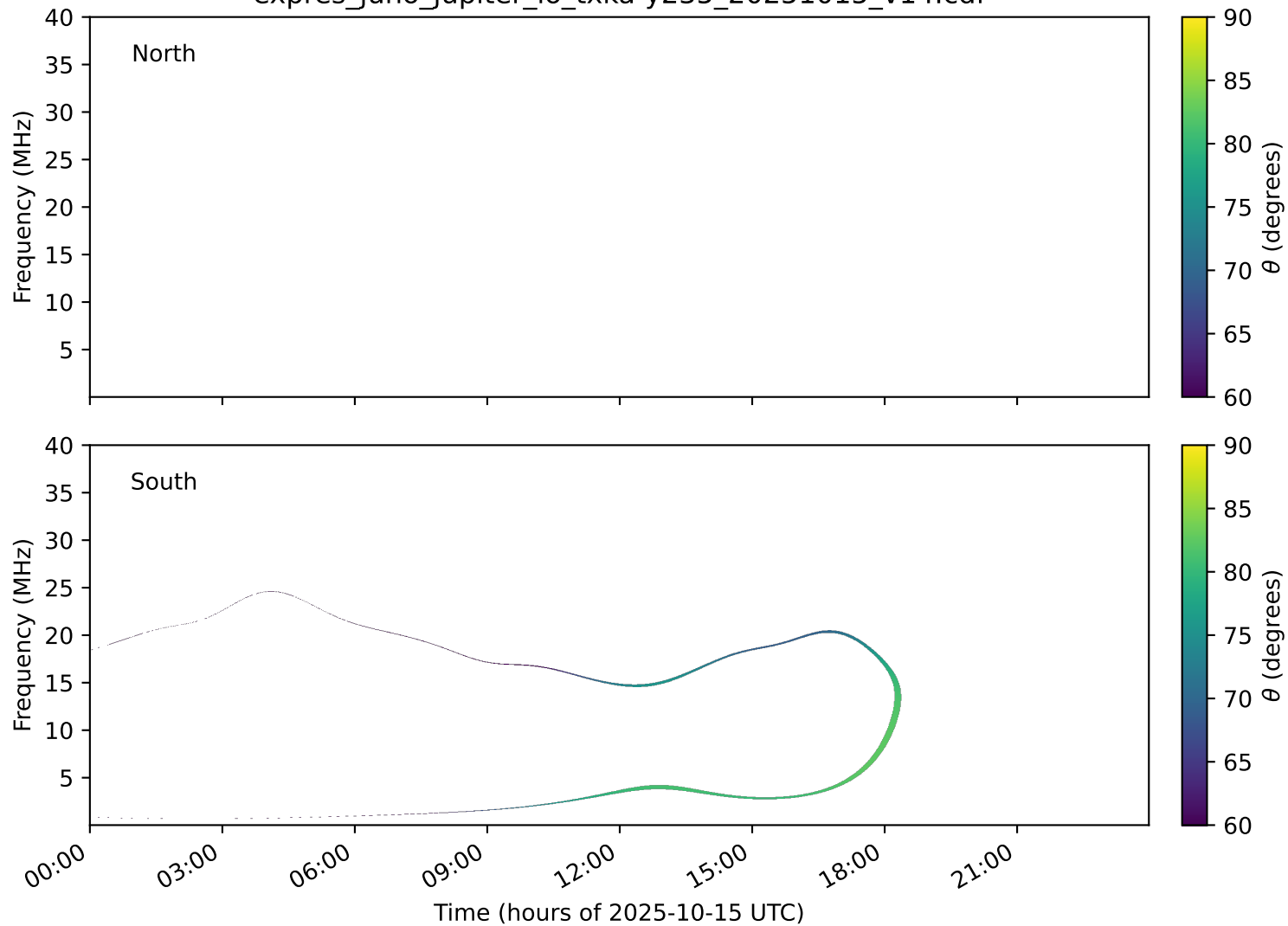
expres_juno_jupiter_io_txka-y235_20251015_v14.cdf
