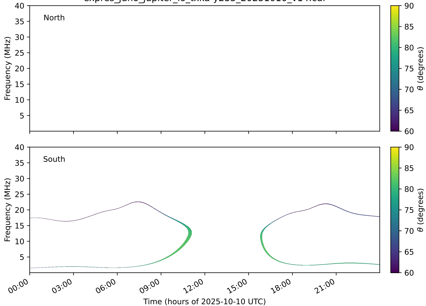
expres_juno_jupiter_io_txka-y235_20251010_v14.cdf
