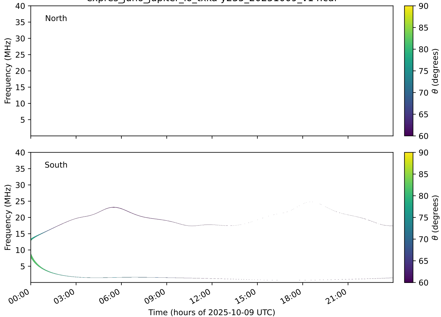
expres_juno_jupiter_io_txka-y235_20251009_v14.cdf
