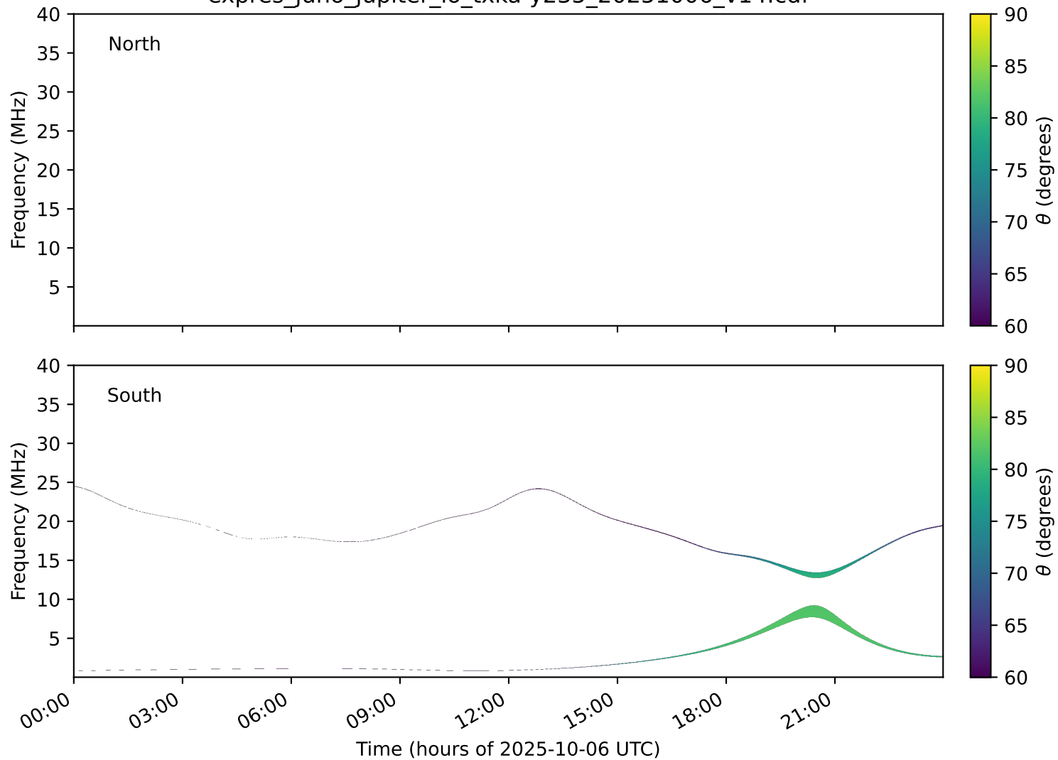
expres_juno_jupiter_io_txka-y235_20251006_v14.cdf
