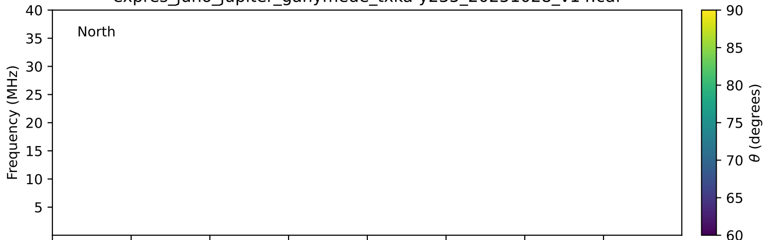
expres_juno_jupiter_ganymede_txka-y235_20251028_v14.cdf
