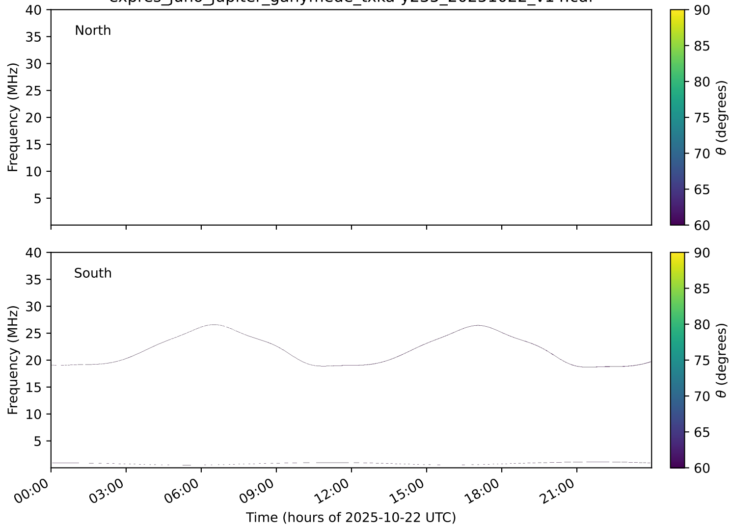
expres_juno_jupiter_ganymede_txka-y235_20251022_v14.cdf
