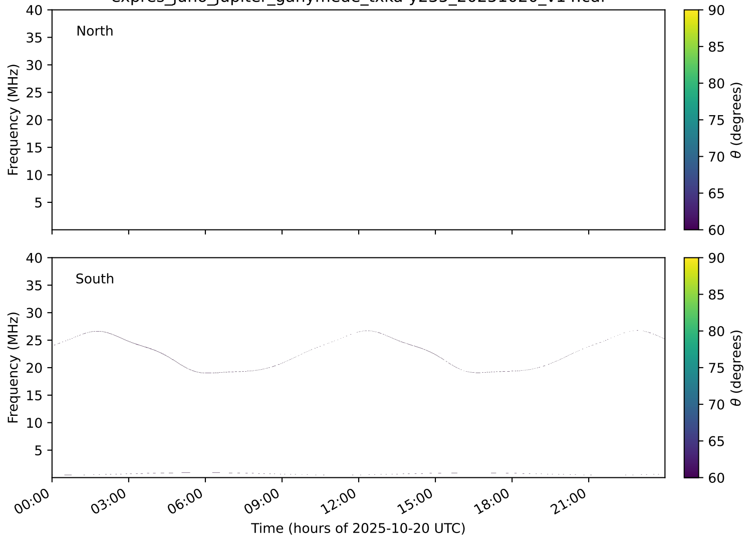
expres_juno_jupiter_ganymede_txka-y235_20251020_v14.cdf
